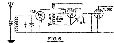
CIRCUIT OF A SUCCESSFUL SET USING THE METHODS DESCRIBED
