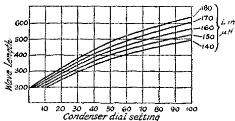
FIG. 4 TUNING CURVES.
