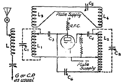
FIG. 2 - IMPROVED MEISSNER CIRCUIT
