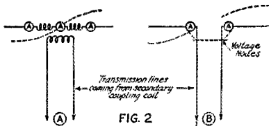
FIG. 2 CURRENT-FEED SYSTEMS
