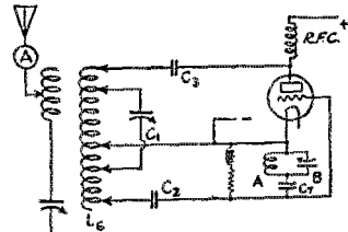
FIG. 4 IMPROVED HARTLEY CIRCUIT
